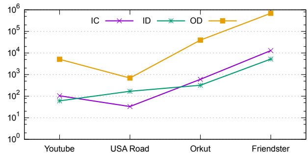
Figure 12: Categorical comparison of PAC for Triangle Counting
