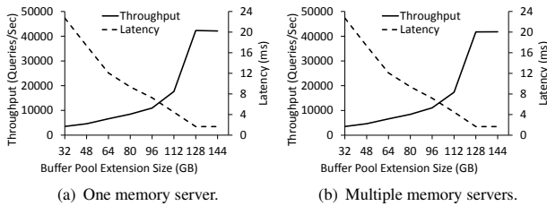
Figure 12: Impact of varying BPExt size.
