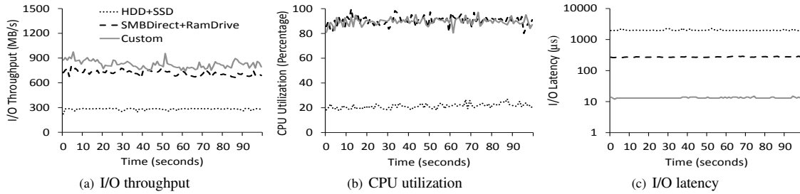
Figure 11: Drill down of RangeScan.
