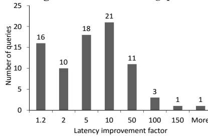
Figure 21: TPC-DS latency improvement.
