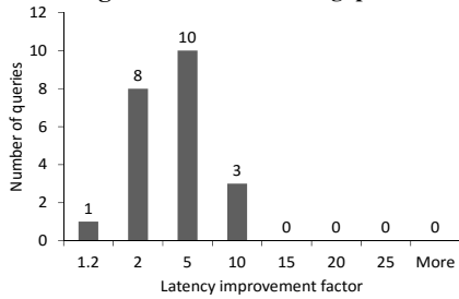
Figure 19: TPC-H latency improvement.
