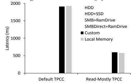
Figure 23: TPC-C latency.
